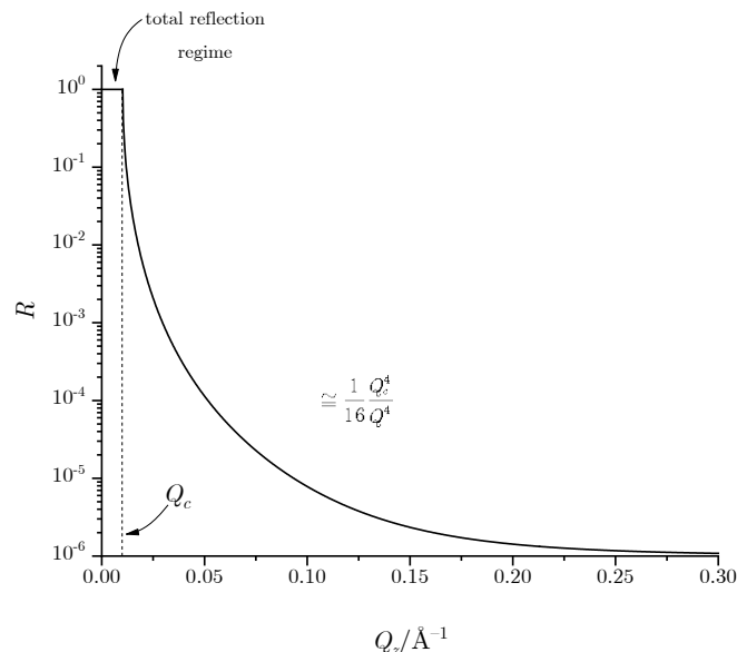
Figure 3 – Theoretical trend of reflectivity of an air/Silicon interface as a function of the modulus of scattering vector. An intrinsic “background” value of 1 \cdot 10^{-6} has been assumed to realistically simulate the curve.
