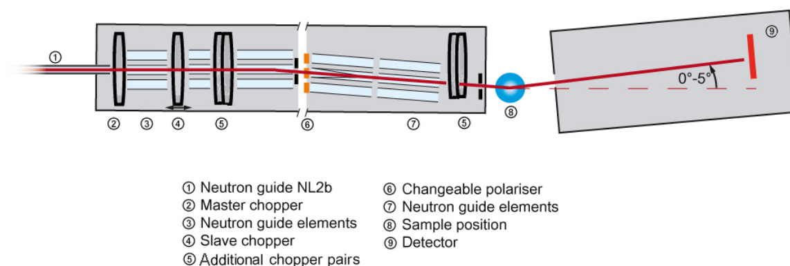
Figure 8 – Sketch of REFSANS as seen from the side.
