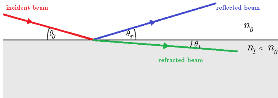
Figure 2 – Reflection and refraction from a smooth surface: \theta_0 is the incident angle, whereas \theta_r = \theta_0 and \theta_1 are the reflection and refraction angles, respectively. n_0 and n_1 indicate the refraction indices: in the figure n_1 < n_0 , so the refracted beam bends outwards.
