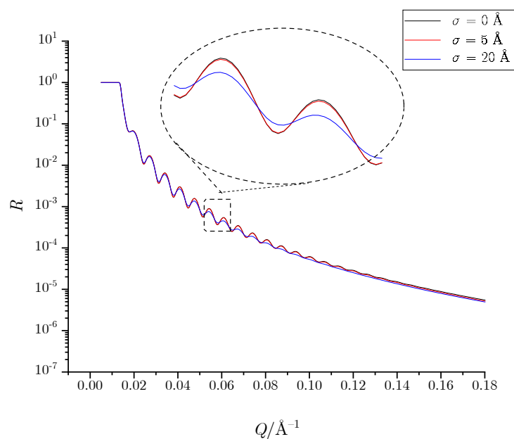
Figure 7 – Theoretical trend of reflectivities for a layered system with air/Titanium/glass interfaces for different values of the air/Titanium interfacial roughness. The inset highlights the different trends.
